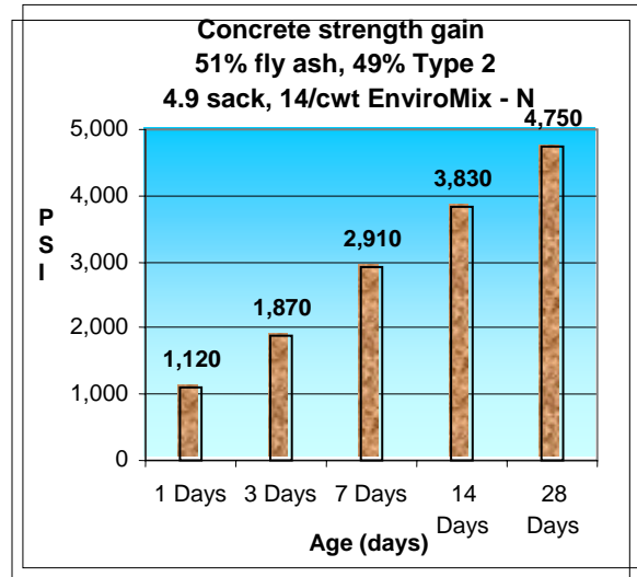
Field results at a 6.5" slump
